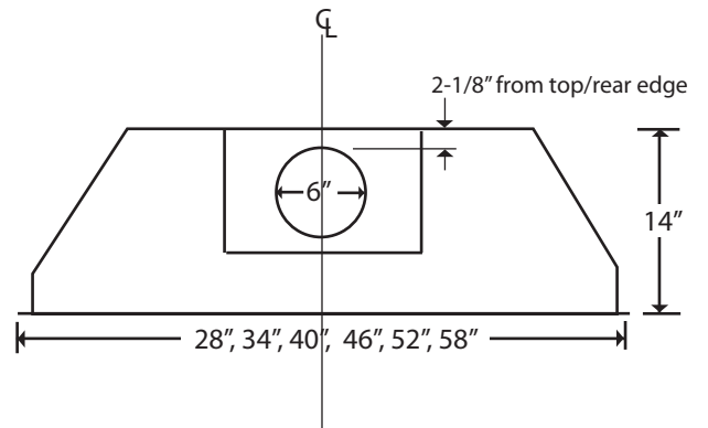
L-Bracket positioned for rear exhaust (Rear View)
